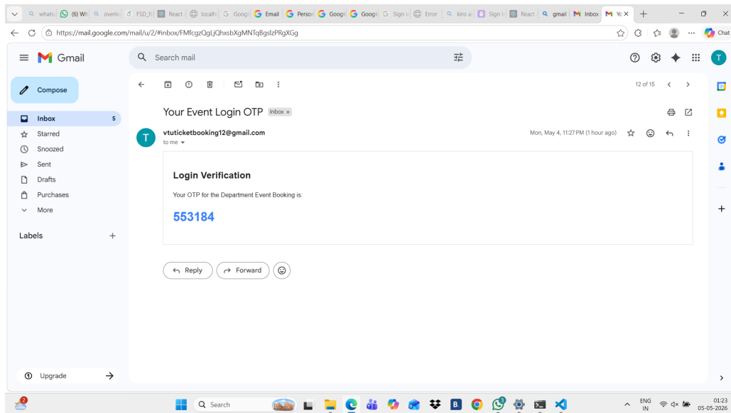
Figure 5.3: Otp Message
