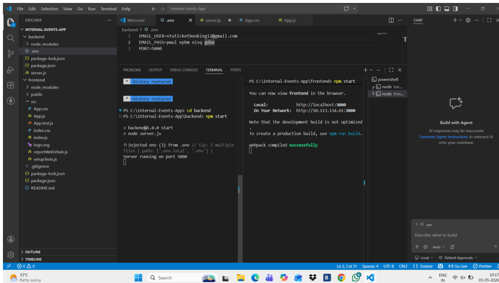
Figure 3.1: Backend Implementation
